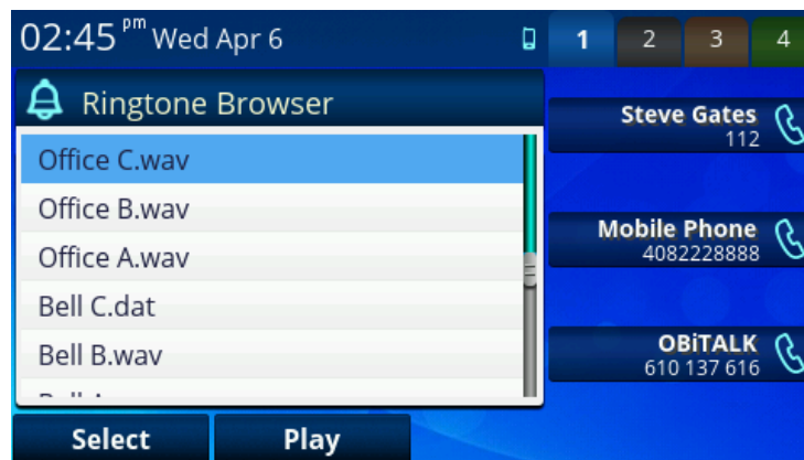
Figure 77: Ringtone browser
