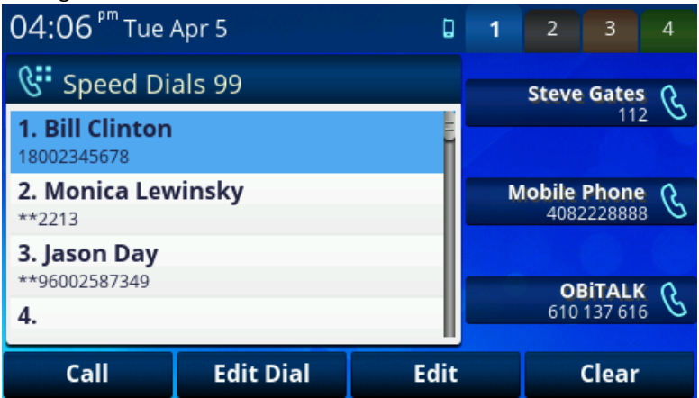
Figure 52: Speed Dials 99
